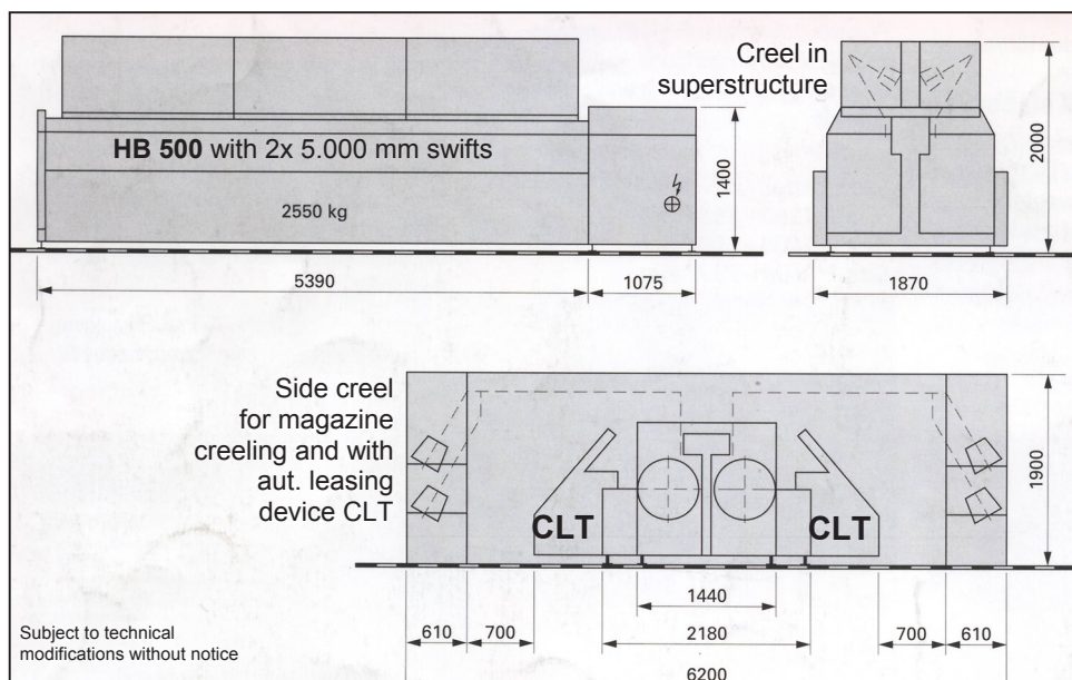
Dimensional drawing (measurements in mm)
